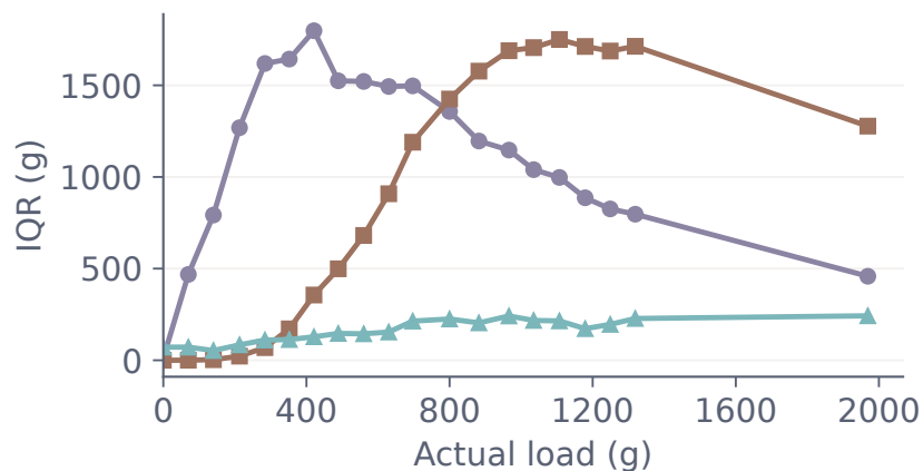
(c) Interquartile range
